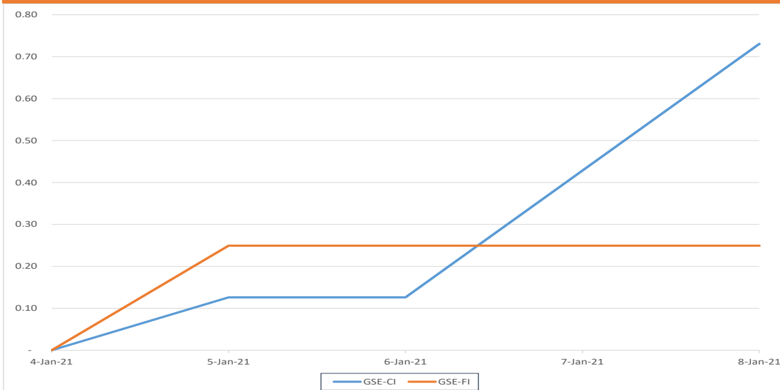
Index YTD Performance (%) as at 8 th January 2021
